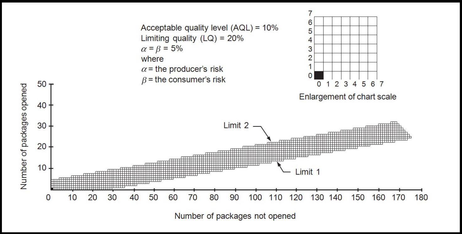
Figure 1/ Figure 1B. Chart of a sequential child-resistant effectiveness test procedure (without demonstration) for reclosable child-resistant packages
