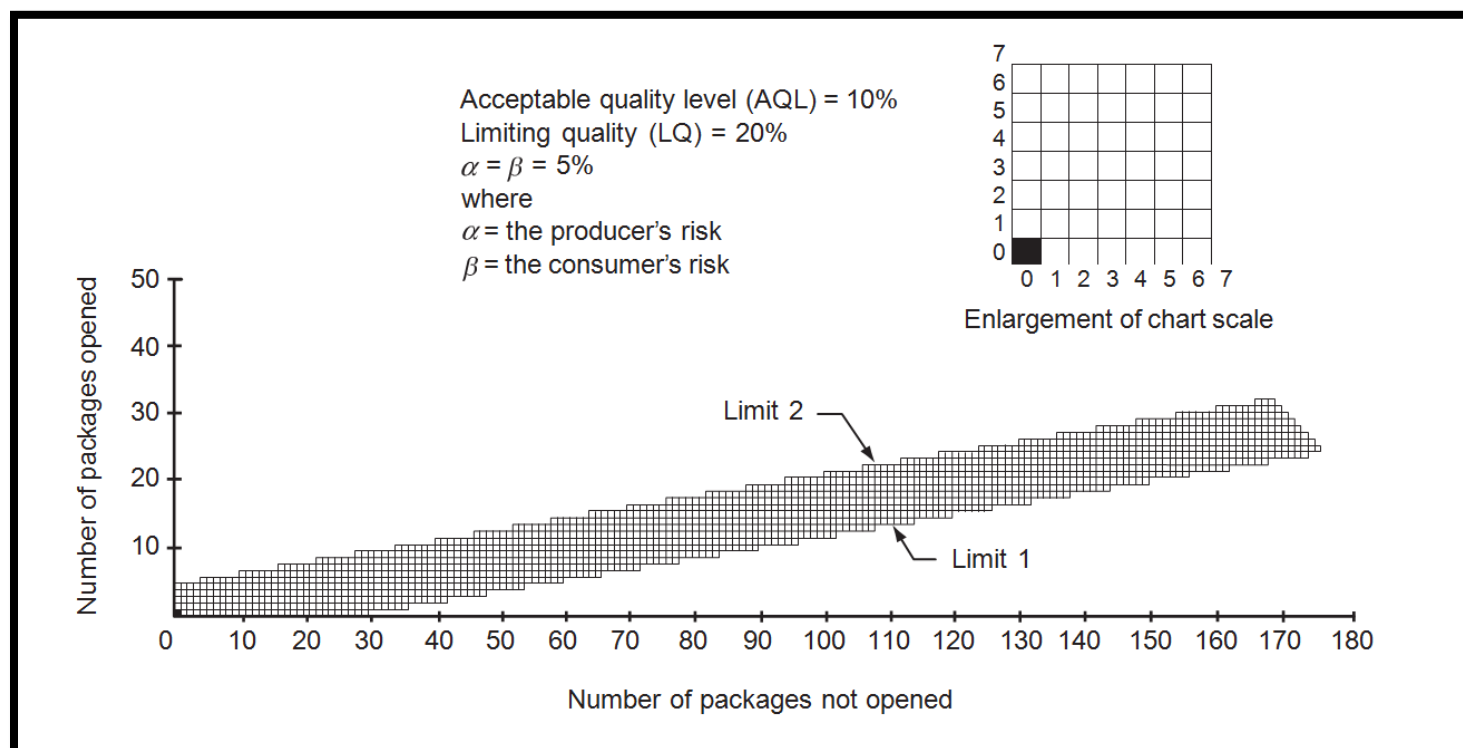
Figure 1/ Figure 1B. Chart of a sequential child-resistant effectiveness test procedure (without demonstration) for reclosable child-resistant packages
