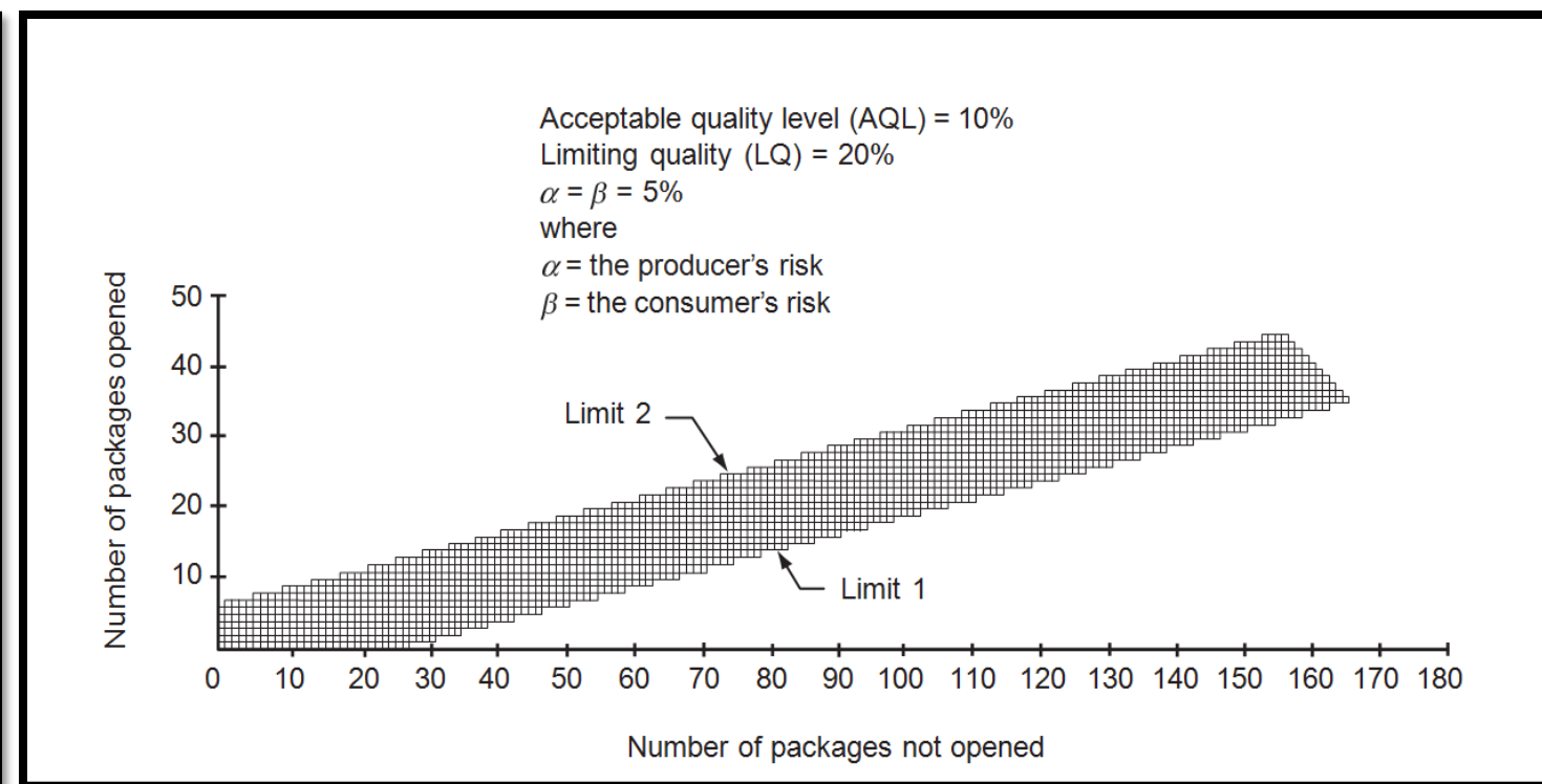
Figure 2 /Figure 2B. Chart of a sequential child-resistant effectiveness test procedure (after demonstration) for reclosable child-resistant packages
